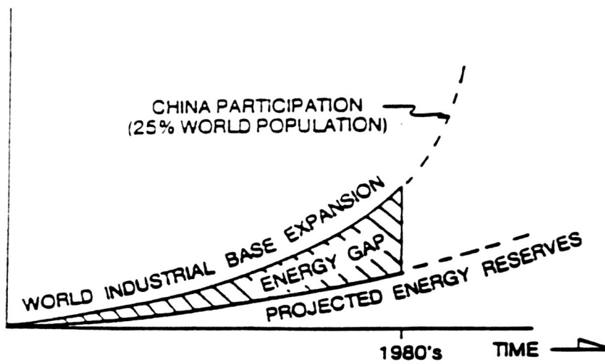
FIG. 1: ENERGY GAP
