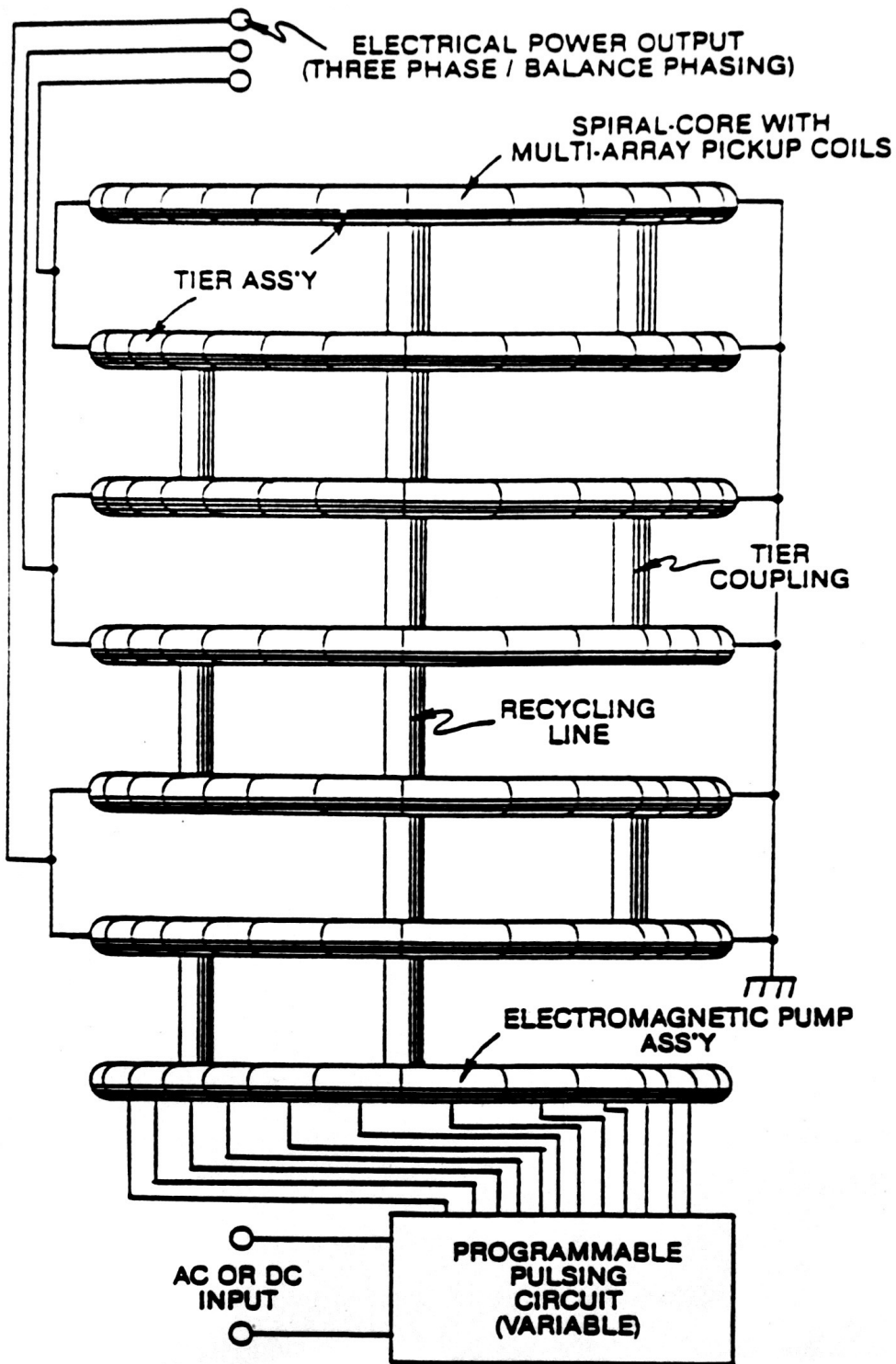
FIG. 26C: MULTI-TIER EPG ELECTRICAL GENERATOR
