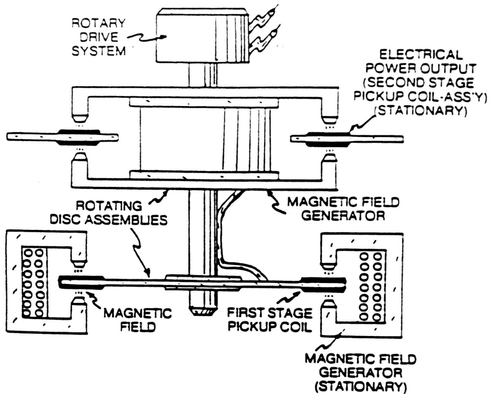
FIG.34: ROTARY PULSE VOLTAGE FREQUENCY GENERATOR
